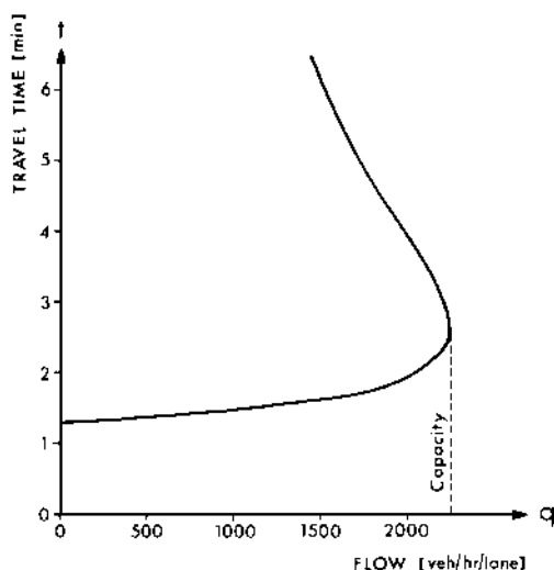
Figure 13.5 Travel time versus flow for Greenshield's speed-density relationships.
