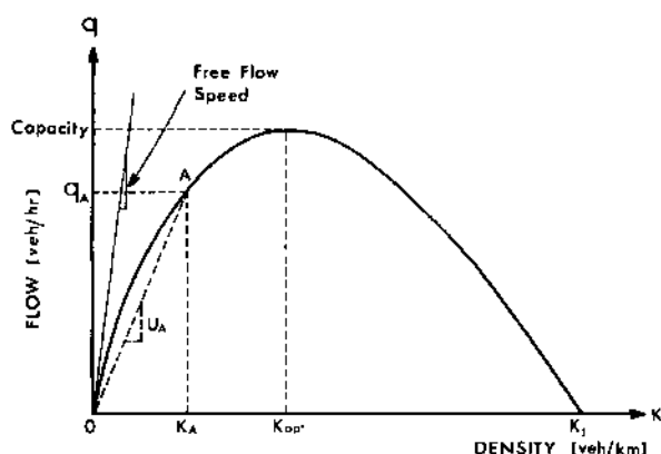
Figure 13.4 Fundamental diagram of traffic flow for a given road segment.
