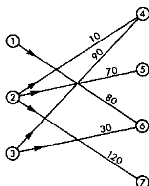
Figure 7.12 Optimal solution of the transportation problem example.
