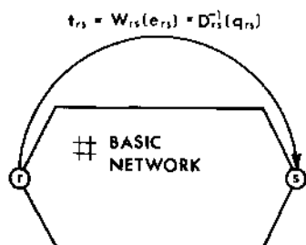
Figure 6.5 Excess-demand network representation for O-D pair r-s .
