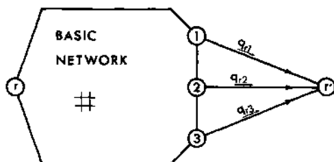
Figure 7.1 Network representation for solving a joint distribution/assignment problem; dummy links are added from each destination node to a new "origin-dummy" node.
