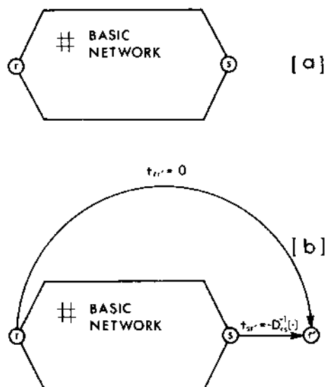
Figure 6.3 The zero-cost overflow network representation: (a) the basic network; (b) the added node and links for O-D pair r-s .
