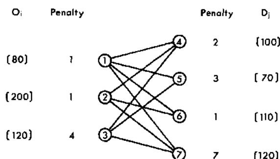
Figure 7.7 The original penalties for the network example. These penalties indicate that link 2 \rightarrow 7 should be examined first. (Node 7 is associated with the highest penalty and link 2 \rightarrow 7 with the lowest cost among all links entering node 7.)
