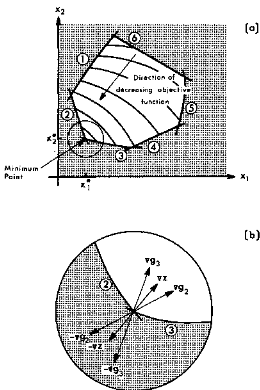
Figure 2.7 Kuhn-Tucker conditions: (a) contours of the objective function and the feasible region; (b) the gradient of the objective function lies within the cone generated by the gradients of the binding constraints.
