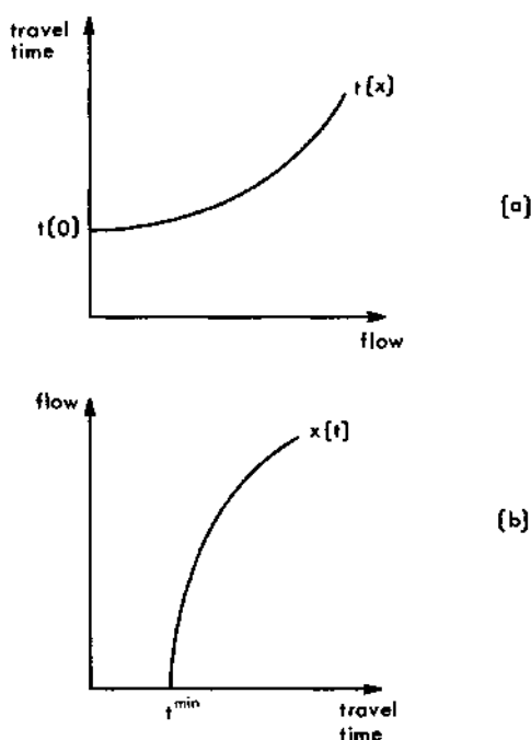
Figure 12.3 Inversion of a link performance function: (a) a link performance function; (b) the inverse of the performance function in (a).
